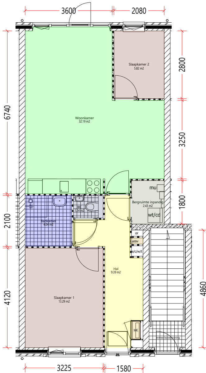
Begane_grond
